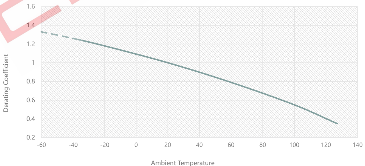
Derating Curve
